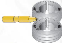
Kit contains 2 drive rolls and 1 inlet guide
