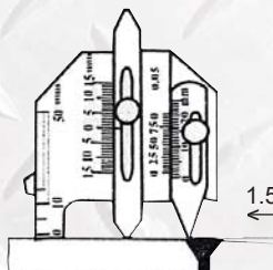
Weld seam undercut depth measurements
