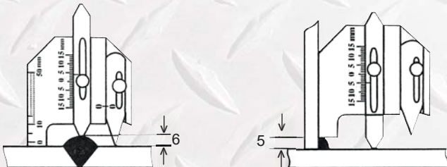
Flat weld height measurements
