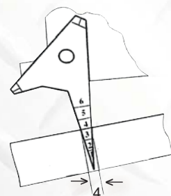
Gap size measurements
