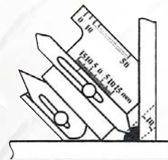
Weld seam undercut depth measurements
