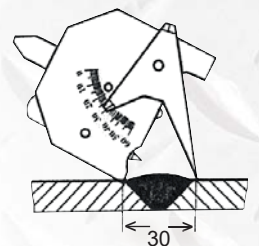
Gap size measurements
