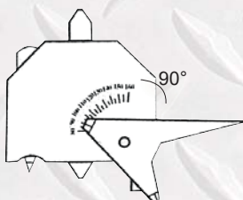
Weldment bevel angle measurements
