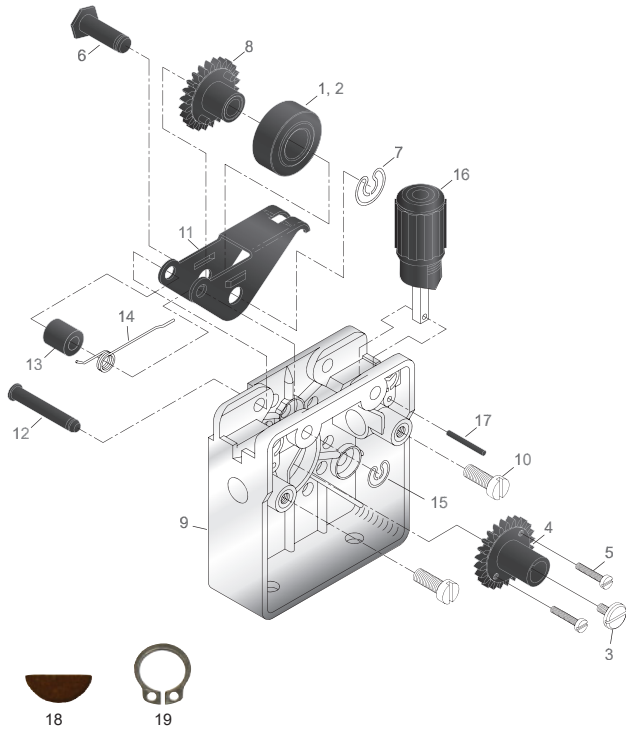
Drive 2 Roll Assembly Breakdown Figure A
