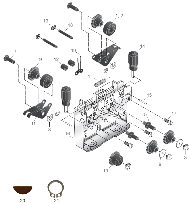
Drive 4 Roll Assembly Breakdown Figure B
